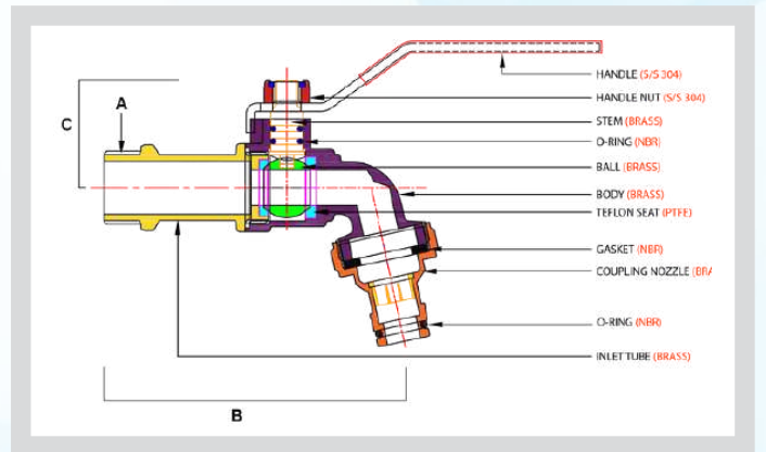
1/2" CP BALL VALVE TAP W/O NOZZLE COUPLING (16MM BALL)
