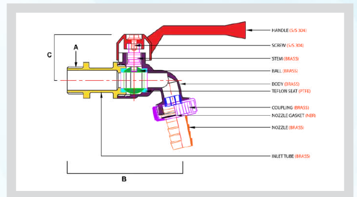
1/2" BALL VALVE TAP WITH NOZZLE COUPLING & O-RING (17MM BALL)
